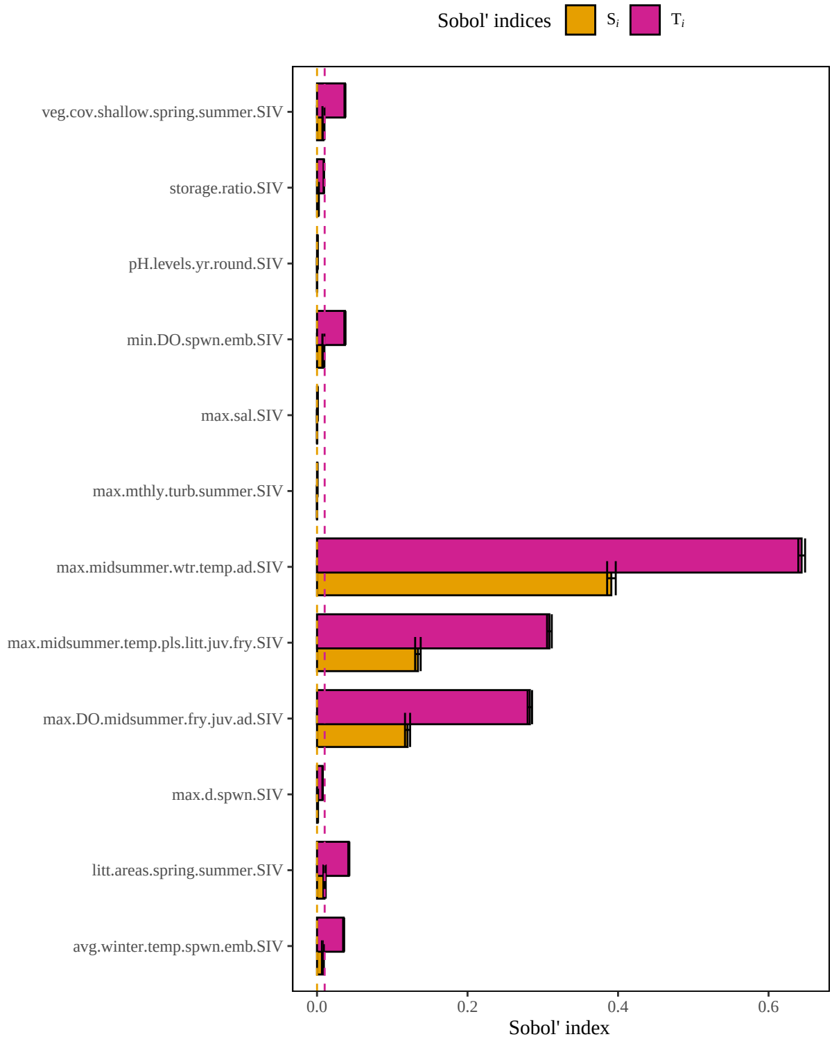
Figure 3. Results of a sensitivity analysis for the commoncarpLacSal model based on the original author-specified model outlined in Edwards and Twomey (1982). Dashed lines represent baseline numerical approximation error for S_i and T_i ( i.e. , dummy variables).
